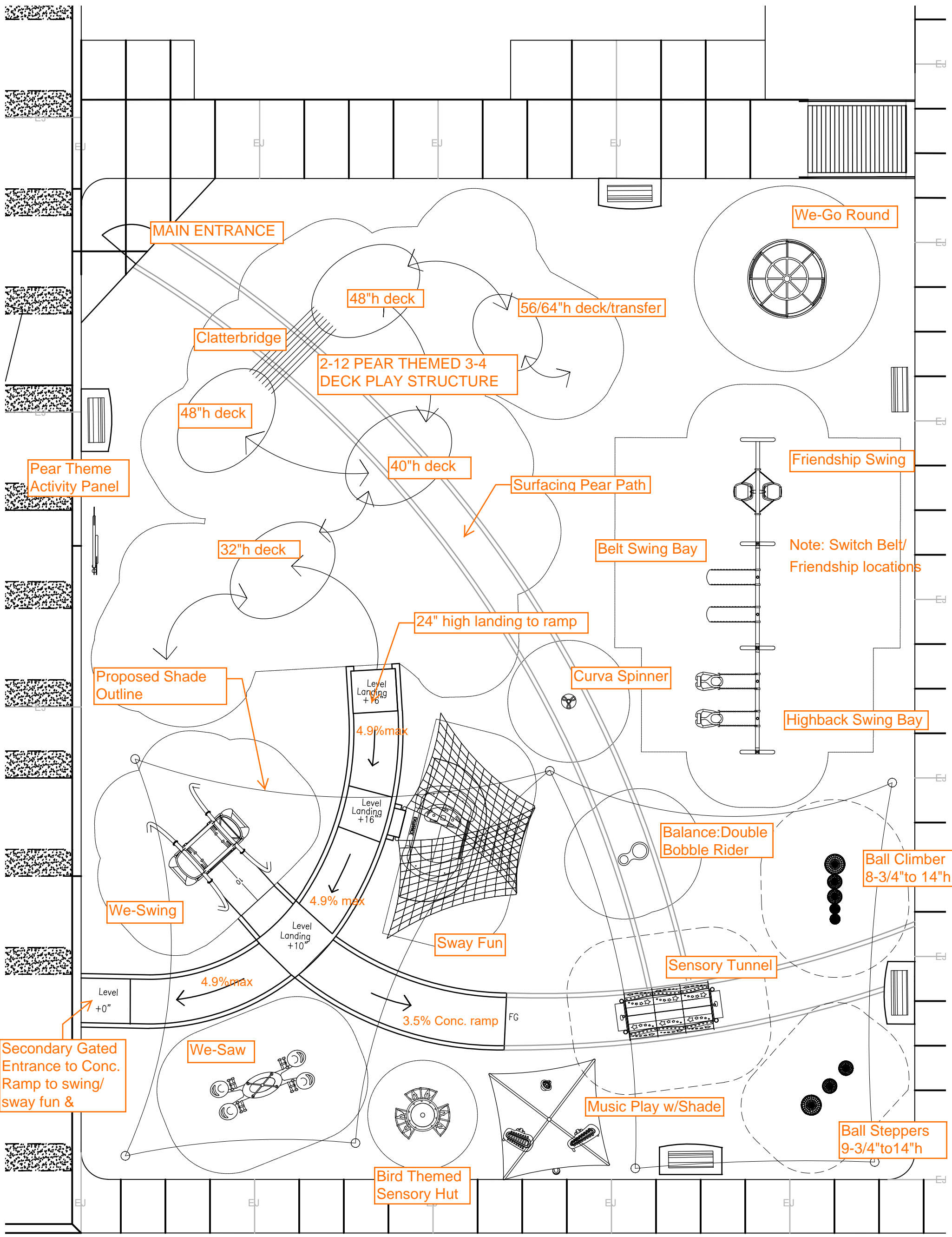
PEARLAND INCLUSIVE PLAYGROUND IMSI CONCEPT PLAN LAYOUT Scale: 1"=10' Date: 2015-02-15
